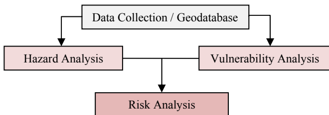
Figure 2: Methodology
