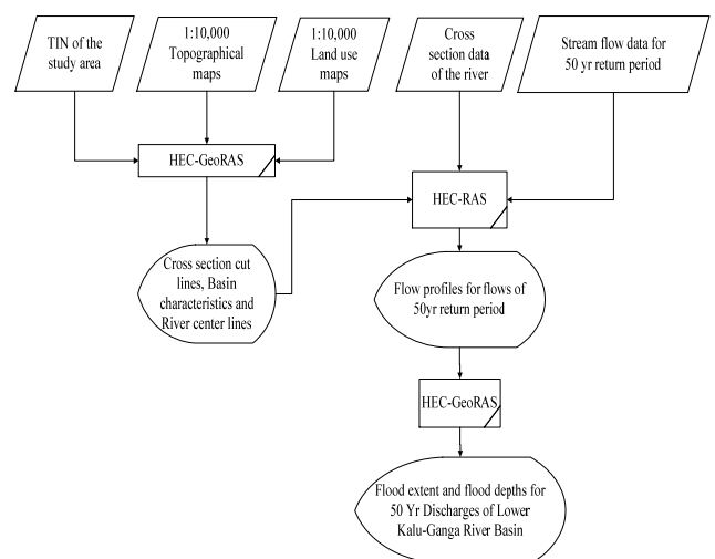
Figure 3: Steps applied for HEC-RAS modeling
